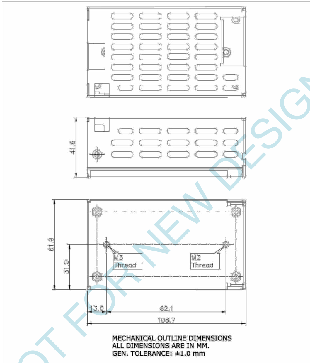
Figure 3. Mechanical Drawing with Cover Kit
