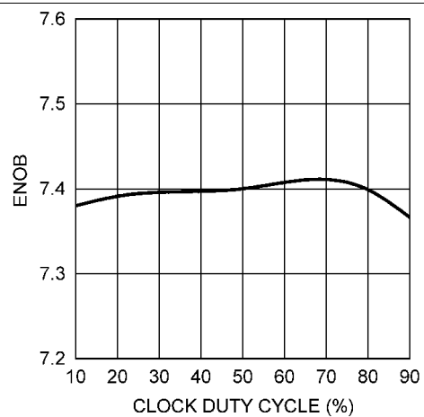
Figure 17. ENOB vs. CLOCK DUTY CYCLE
