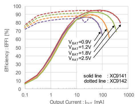
XC9141A33C / XC9142A33C L=4.7µH(LQH5BPN4R7NT0L) C_{IN}=10\mu F (GRM188R60J106M), C_L=10\mu F (GRM188R60J106M)
