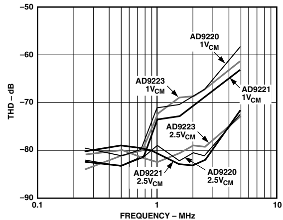
Figure 6. AD9221/AD9223/AD9220 THD vs. Frequency for V_{CM} = 2.5\text{ V} and 1.0\text{ V} ( A_{IN} = -0.5\text{ dB} , Input Span = 2.0 V p-p)
