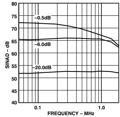
TPC 6. SINAD vs. Input Frequency (Input Span = 5.0 V p-p, V_{\text{CM}} = 2.5 \text{ V} )
