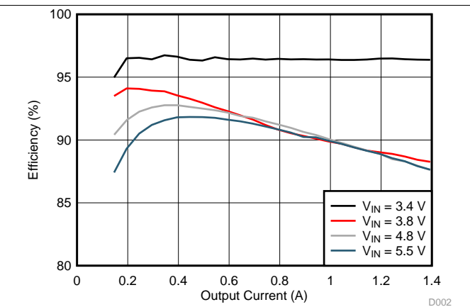
Figure 3. PWM Efficiency vs Output Current
