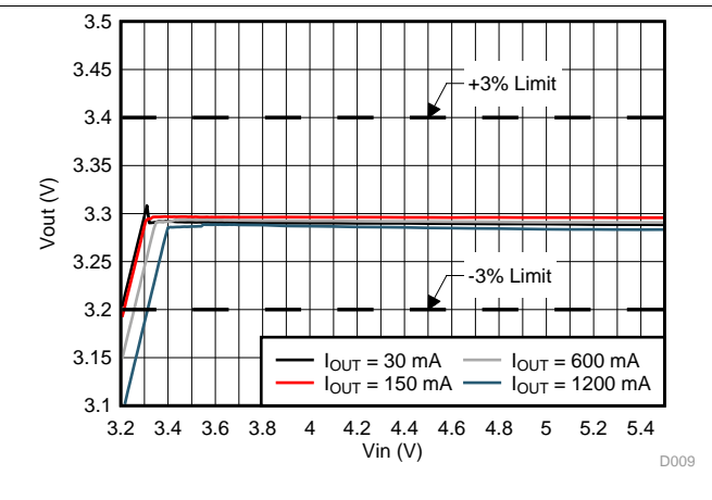
Figure 15. Line Regulation vs Output Current
