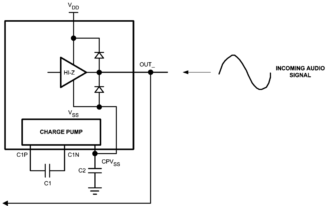
FIGURE 5. Back-Driving the LM48822 Outputs
