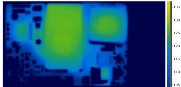
Figure 4. Thermal Image of CPT1U48 1.25A output, 55C Ambient, 200lfm airflow, Vin = 48V, airflow from pin 3 to pin 1, T max = 125°C
