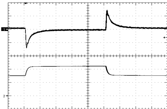
Figure 9. Load Transient Response (100mV/div), di/dt=0.1A/uS, 50% - 75% - 50% of full load, time scale: 200uS/div Ch2=0.5A/div
