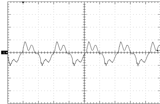
Figure 5. Output Voltage Ripple (100mV/div), time scale – 1uS/div. Vin=Vin_nom, full resistive.
