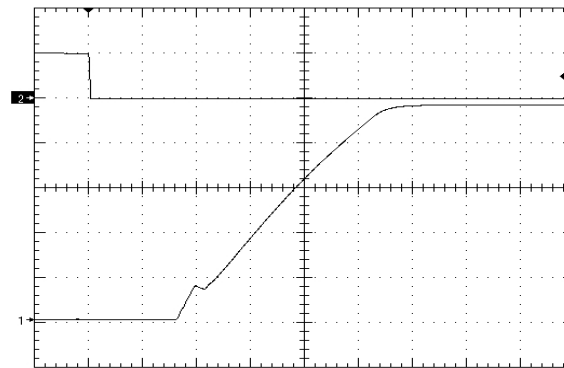
Figure 8. Startup Waveform via Enable Pin, time scale 10mS/div. Vin=Vin_nom, full res. load + 270uF, negative enbl, Ch1=10V/div, Ch2=5V/div
