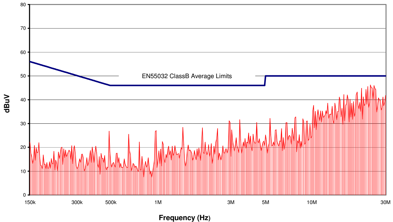
Figure 16. CPT1U48 Conducted Emissions using above specified input filter, Vin = 48V, Full Resistive Load
