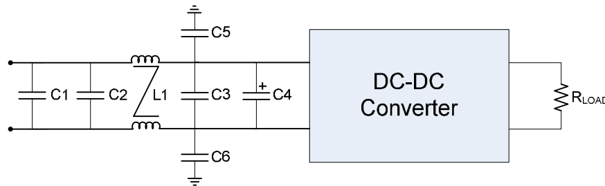
Figure 15. EMI Filter
