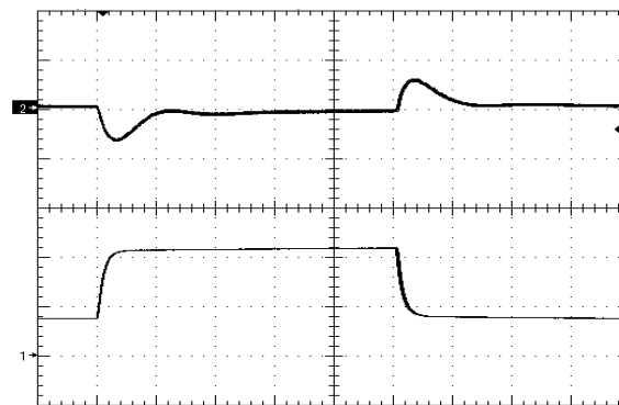
Figure 10. Load Transient Response (100mV/div), di/dt=0.1A/uS, 25% - 75% - 25% of full load + 10uF time scale: 200uS/div Ch1=0.5A/div
