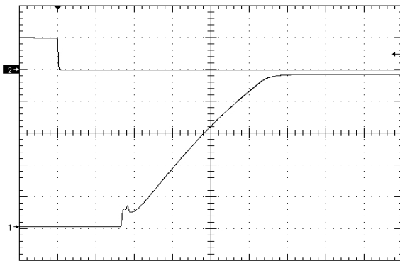
Figure 7. Startup Waveform via Enable Pin, time scale 10mS/div. Vin=Vin_nom, full load Ch1=10V/div, Ch2=5V/div
