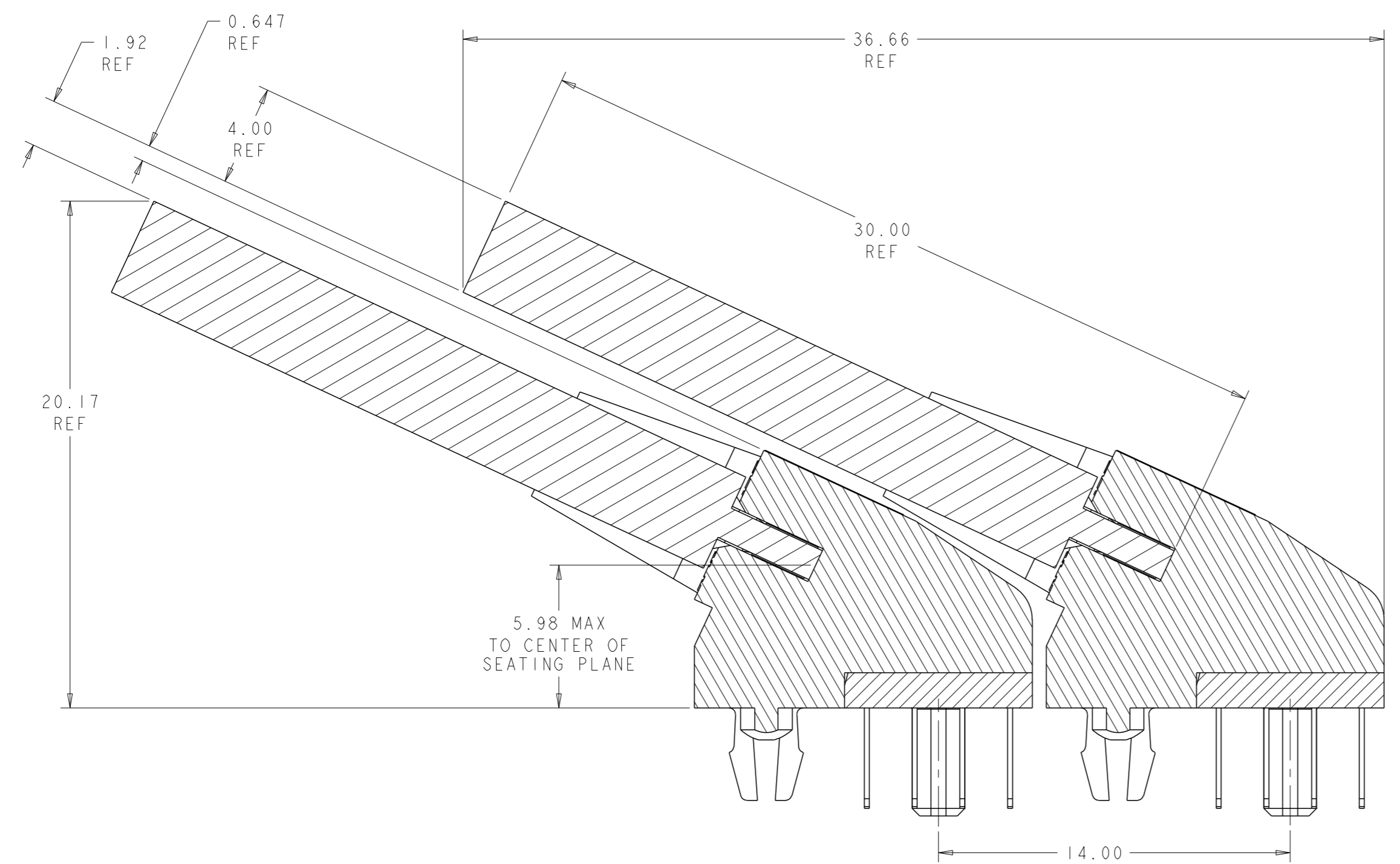
MINIMUM RECOMMENDED ROW TO ROW SPACING FOR 4mm THICK MODULE
