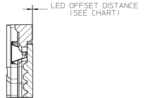
DETAIL 1 SCALE 4:1
