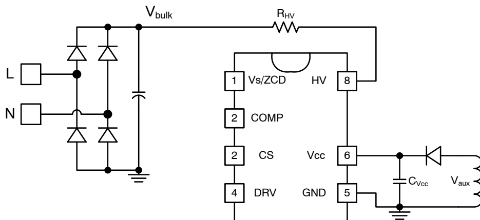
Figure 44. HV Startup Connection to the Bulk Capacitor
