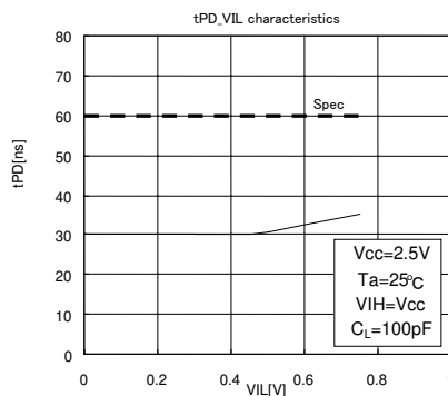
Figure 53. VIL dependency of data output delay time tPD
