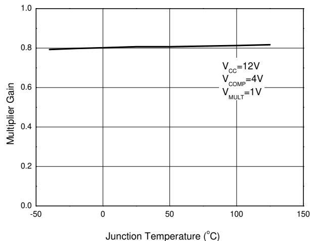
Multiplier Gain vs. T_J
