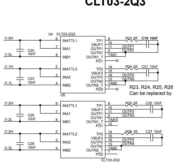
Figure 4. STEVAL-PLC001V1 circuit schematic (3 of 9)
