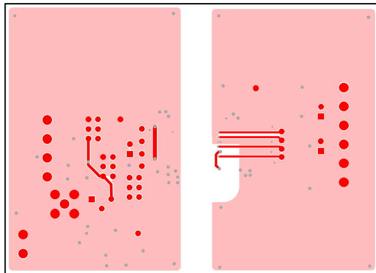
Figure 13. Bottom Layer
