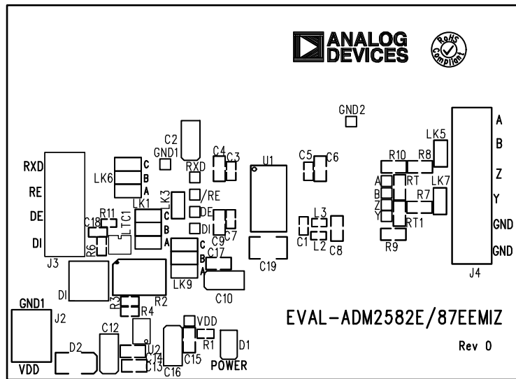
Figure 12. Silkscreen
