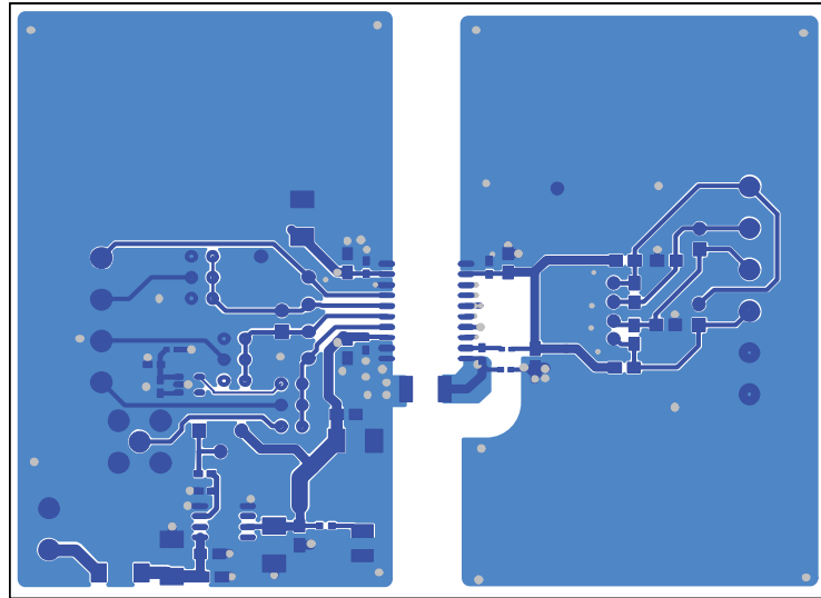
Figure 11. Top Layer
