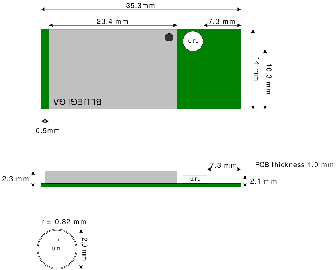
Figure 32: WT11-E dimensions
