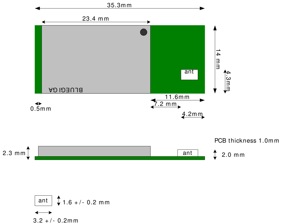
Figure 31: WT11-A dimensions
