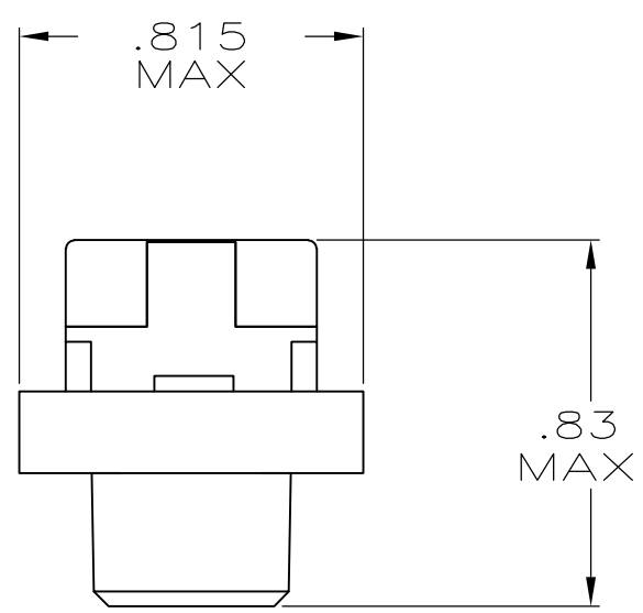
END VIEW
