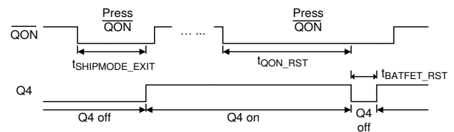
Figure 2. QON Timing
