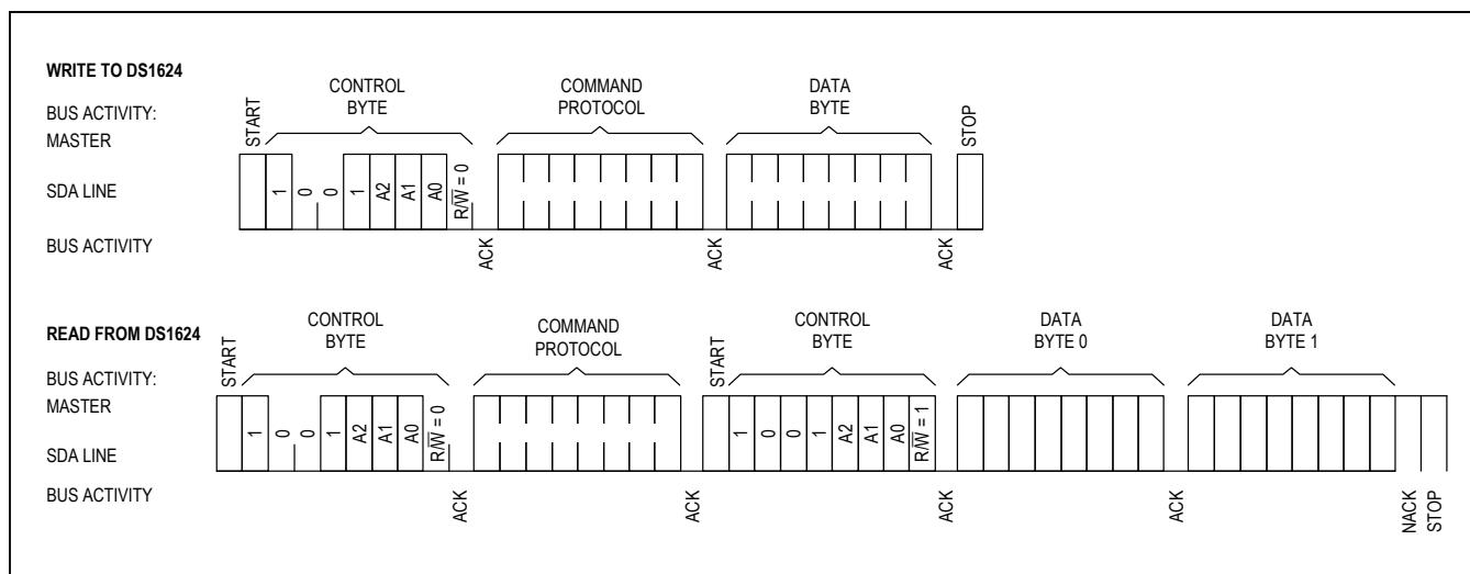
Figure 3. 2-Wire Serial Communication with DS1624
