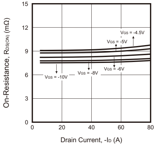
Fig.7 - On-Resistance vs. Drain Current
