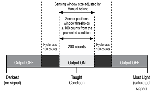
Figure 5. Single-Point Window SET and Hysteresis (Light Operate shown)
