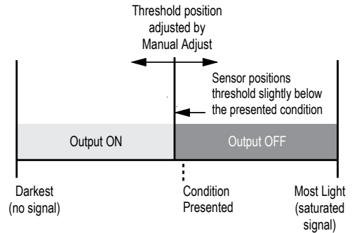
Figure 6. Single-Point Light Set (Light Operate shown)
