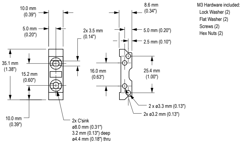
Figure 9. Included bracket dimensions
