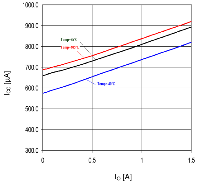
Figure 32. I o -I cc
