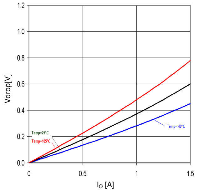
Figure 34. Minimum dropout Voltage 2 (V CC =4.5V、T a =25°C)
