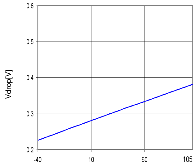
Figure 30. Minimum dropout Voltage1 (Vcc=6V, Io=1.0A)
