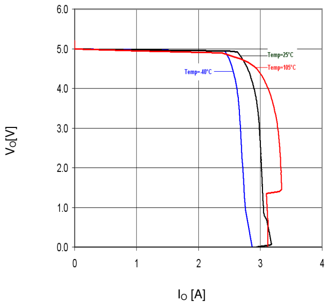
Figure 29. Io-Vo
