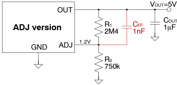
Figure 56. ADJ Output Voltage Schematic – C_{FF} Capacitor
