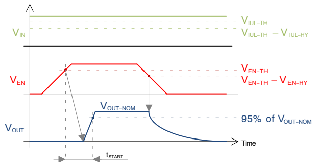
Figure 67. Timing – V_{EN} -Startup
