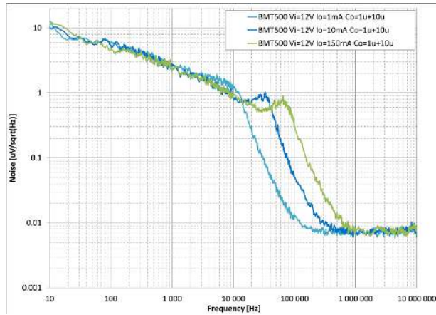
Figure 48. Noise – FIX – 5.0 V, C_{OUT} = 1\text{ }\mu\text{F} + 10\text{ }\mu\text{F} , Different I_{OUT}
