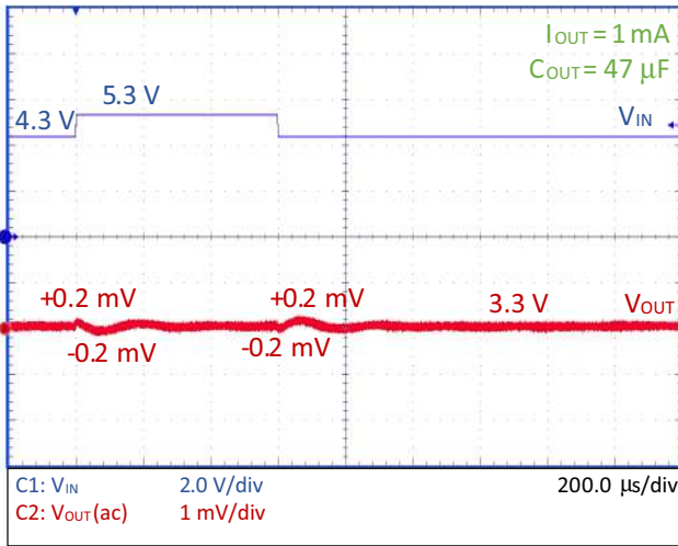
Figure 36. Line Transient – NCP730–3.3 V
