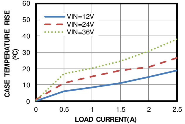
Case Temperature Rise vs. Load Current V OUT = 5V, f sw = 500kHz
