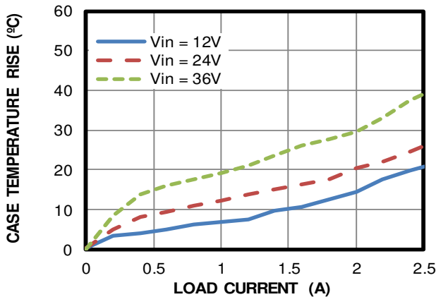
Case Temperature Rise vs. Load Current V OUT = 5V, f sw = 1MHz
