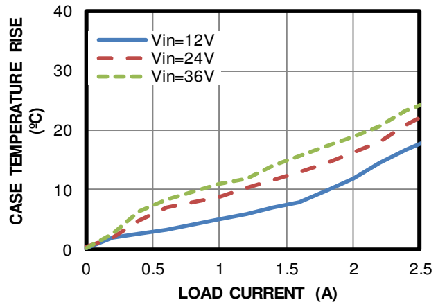
Case Temperature Rise vs. Load Current V OUT = 5V, f sw = 2.2MHz
