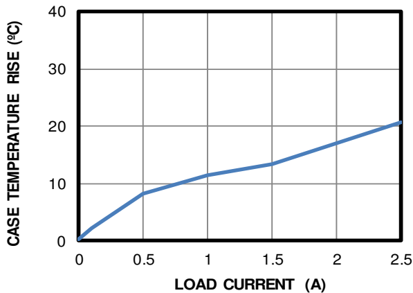
Case Temperature Rise vs. Load Current V OUT = 5V, f sw = 1MHz
