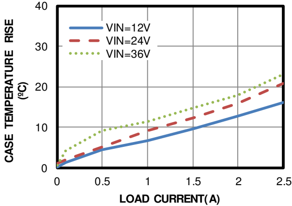
Case Temperature Rise vs. Load Current V OUT = 3.3V, f sw = 2.2MHz
