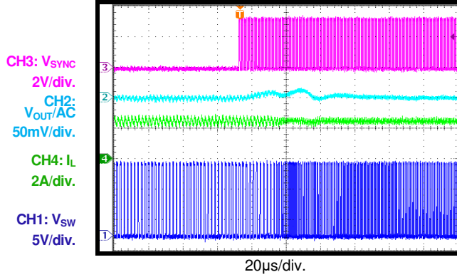
SYNC In Transient
