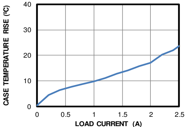
Case Temperature Rise vs. Load Current V OUT = 5V, f sw = 2.2MHz
