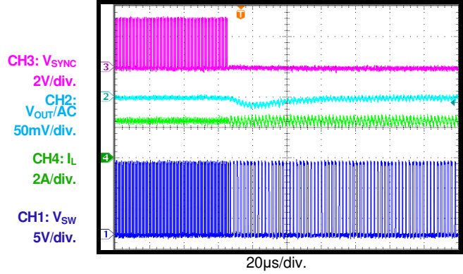
SYNC Out Transient
