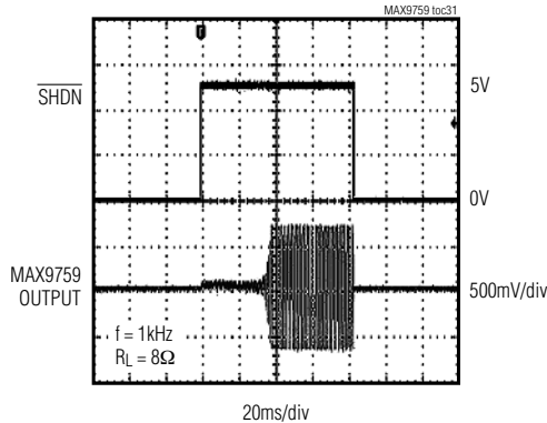
SHUTDOWN RESPONSE
