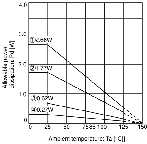
Figure 55. Thermal Derating Characteristics (VQFN016V3030)
