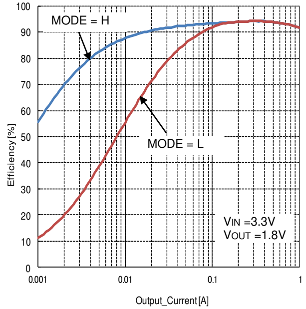
Figure 23. Efficiency vs Load Current (VIN=3.3V, VOUT=1.8V, L=2.2μH)
