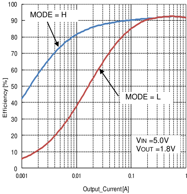
Figure 22. Efficiency vs Load Current (VIN=5V, VOUT=1.8V, L=2.2μH)
