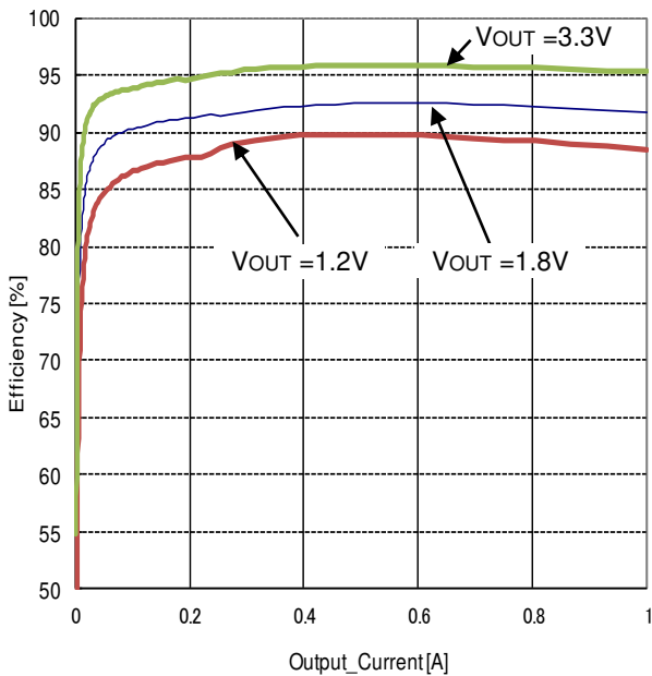
Figure 24. Efficiency vs Load Current (VIN = 5.0V, MODE = 5.0V, L=2.2μH)
