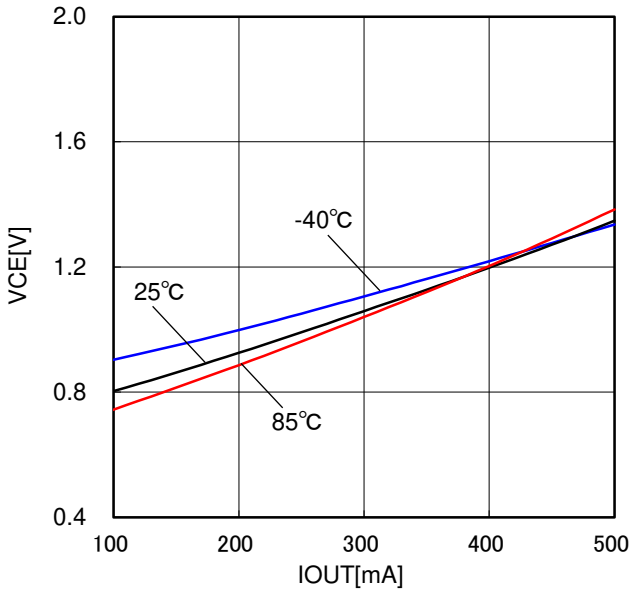
Figure 5 . Output Saturation Voltage2 vs Output Current
