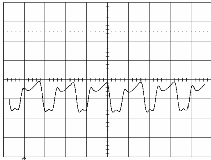
Output voltage ripple (20mV/div.) at: T_{ref} = +25^\circ\text{C} , I_O = 22\text{ A} resistive load, V_i = 3.3\text{ V} . Time scale: 2 \mu\text{s}/\text{div} . See the filter in the Output ripple and noise section (EMC Specification).
