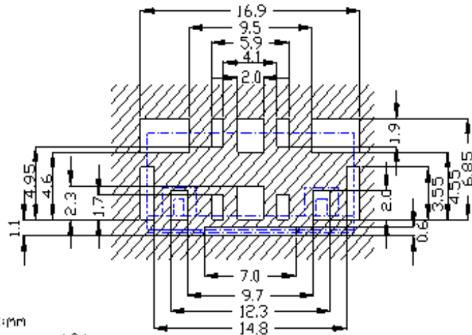
3-2-2 Solder resist Pattern
