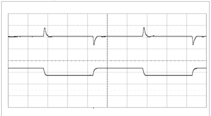
Output voltage response to load current step change (1.5-4.5-1.5 A) at V_I = 12\text{ V} , C_O = 3 \times 100\ \mu\text{F} + 270\ \mu\text{F}/10\text{m}\Omega . Default compensation settings. Scale: 50 mV/div, 5 A/div, 100 \mu\text{s} /div.
