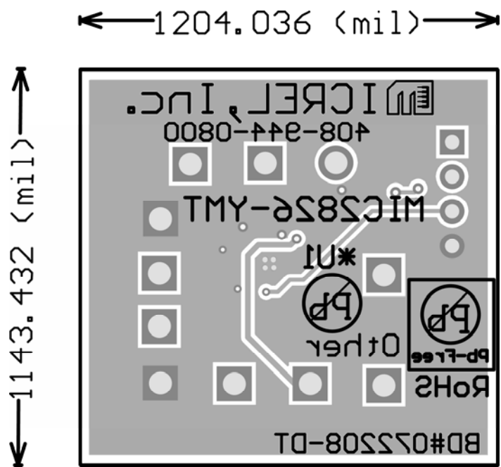
Bottom Layout
