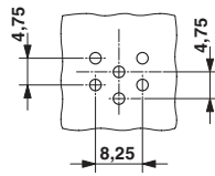
Drilling diagram
