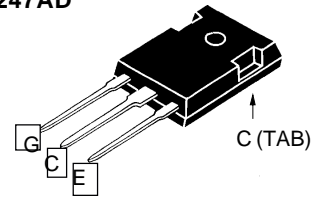
TO-247AD
