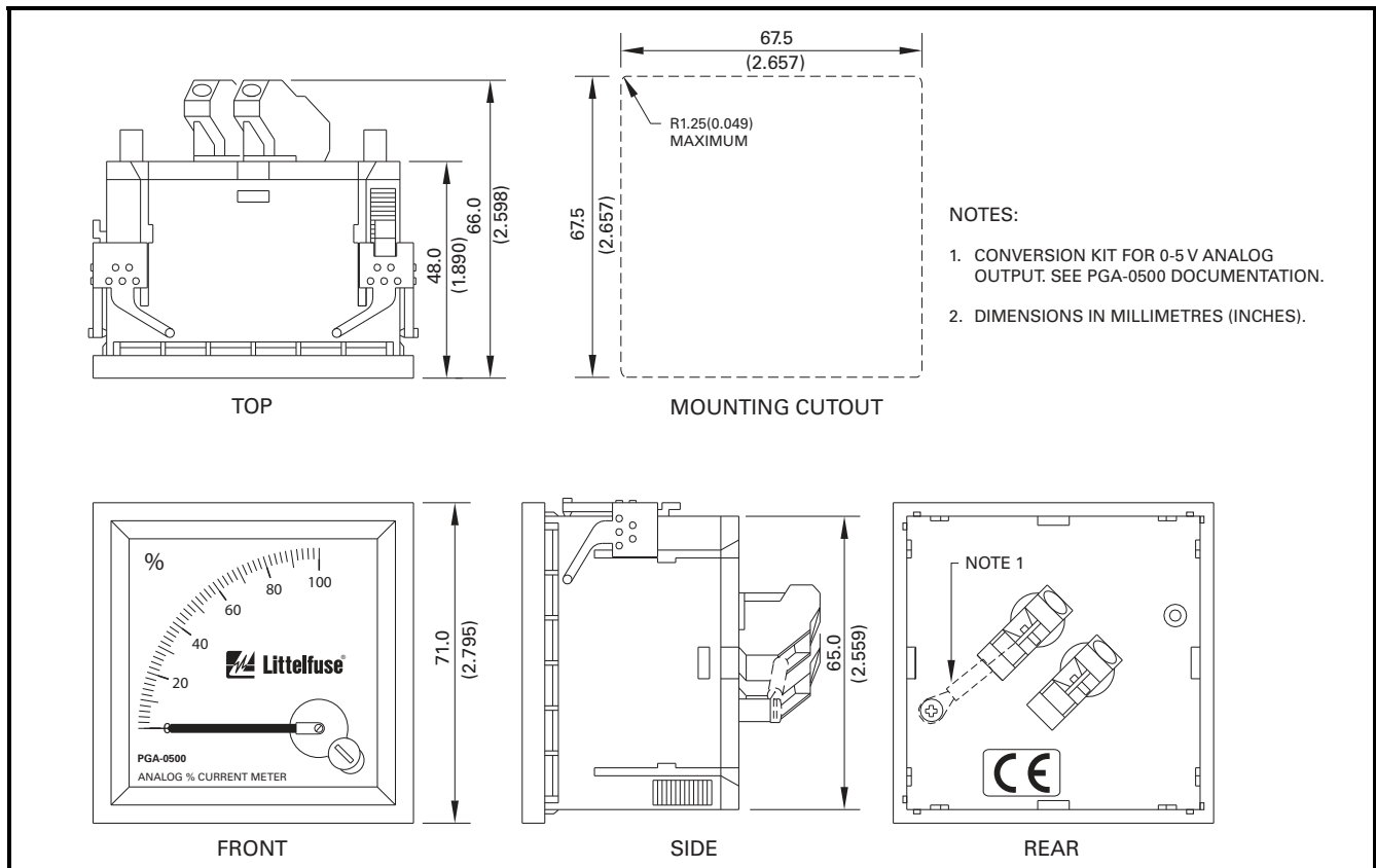
FIGURE 11. PGA-0500 Analog Percent Current Meter.
