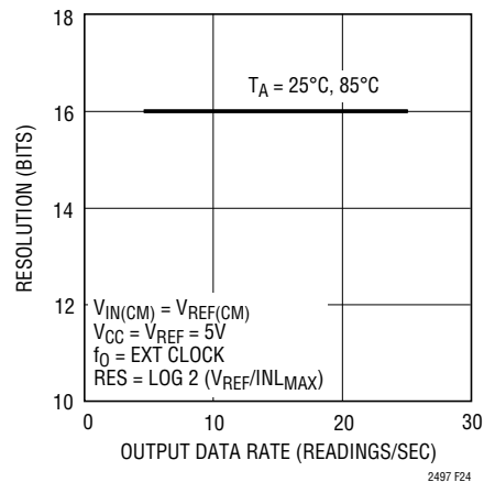
Figure 24. Resolution ( \text{INL}_{MAX} \leq 1\text{LSB} ) vs Output Data Rate and Temperature
