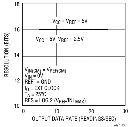
Figure 27. Resolution ( \text{INL}_{MAX} \leq 1\text{LSB} ) vs Output Data Rate and Reference Voltage
