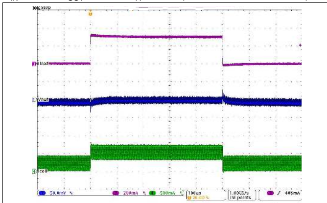
Figure 26. Load Transient Response in PWM Mode (200 mA to 500 mA)
