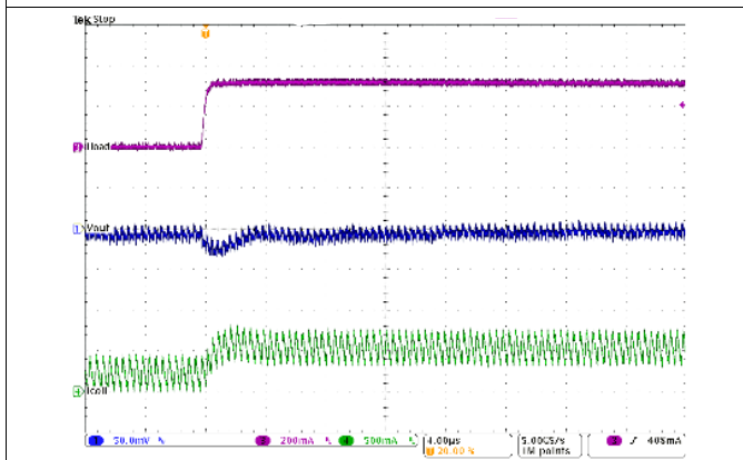
Figure 28. Load Transient Response in PWM Mode (200 mA to 500 mA), Rising Edge
