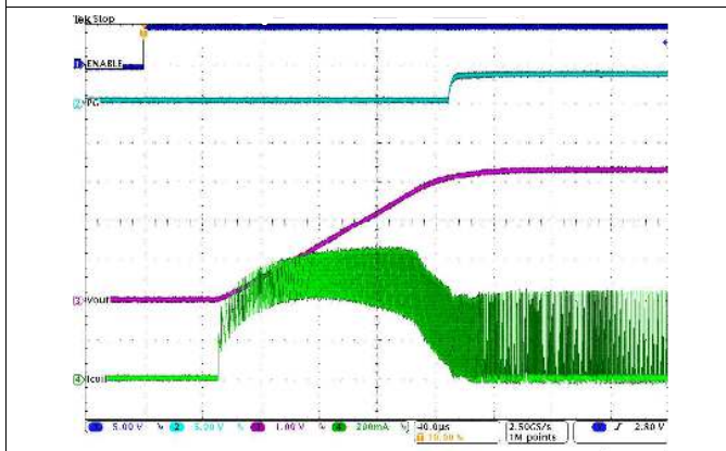
Figure 30. Startup with I_{OUT} = 500\text{ mA} , V_{OUT} = 3.3\text{ V}
