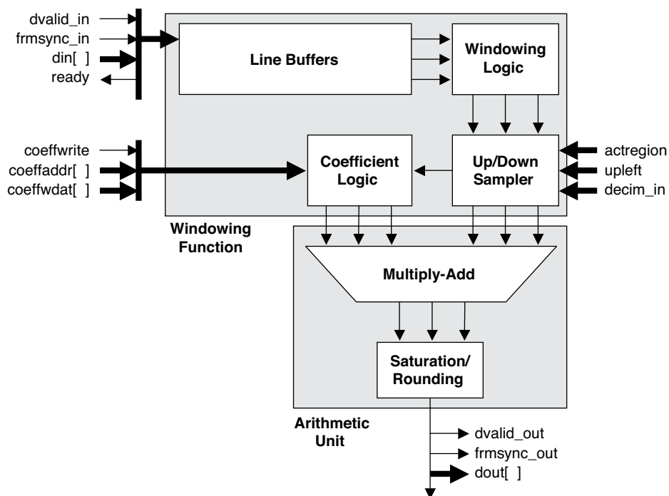
Figure 2-1. 2D FIR Filter IP Core Block Diagram
