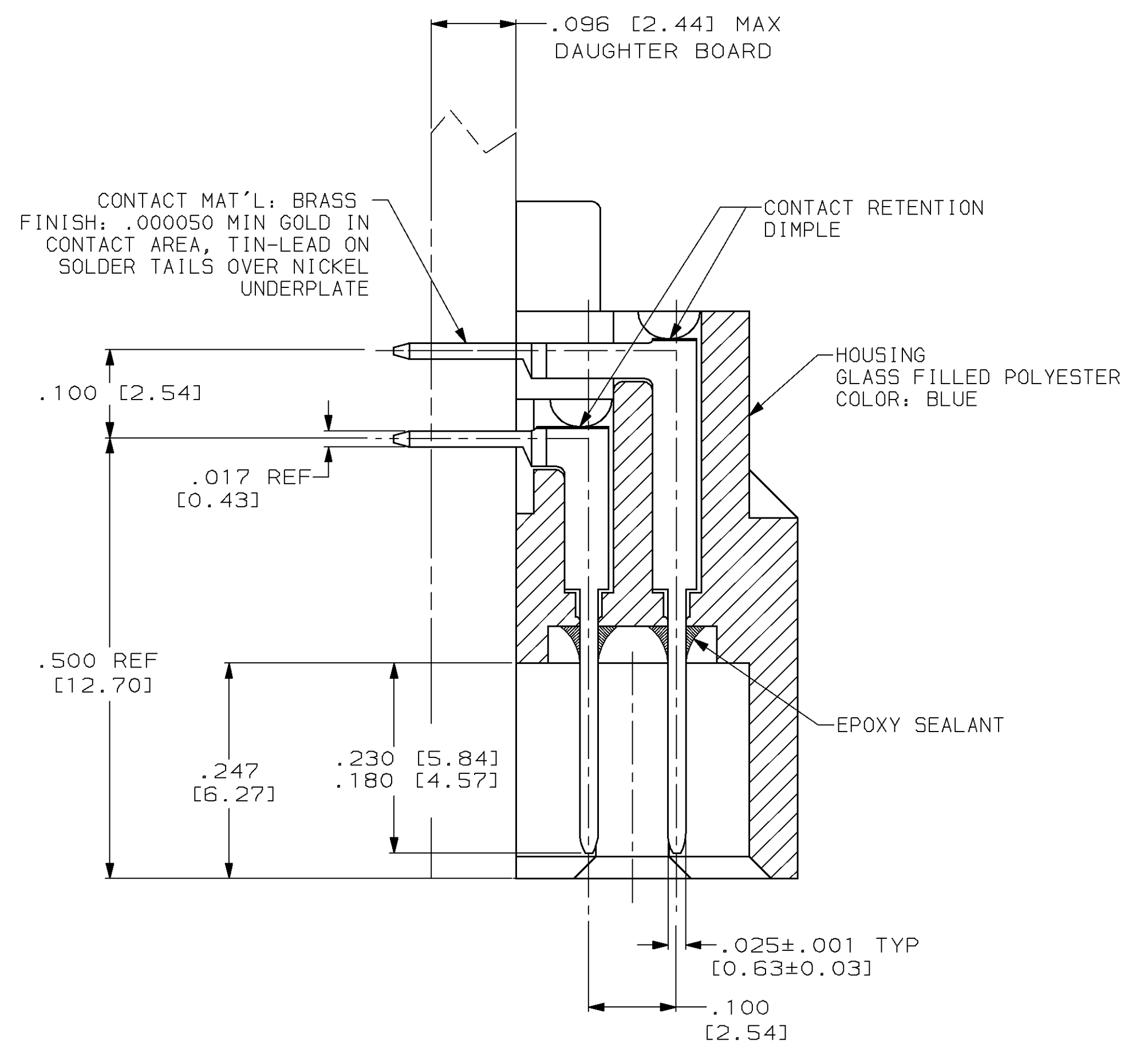
SECTION Y-Y SCALE 8:1
