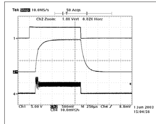
Start up from SHDN, V_{IN} = 5\text{V} , I_{OUT} = 0.4\text{A} , V_{OUT} = 1.5\text{V}
