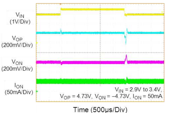
V ON Line Transient
