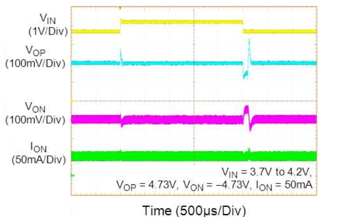
V ON Line Transient
