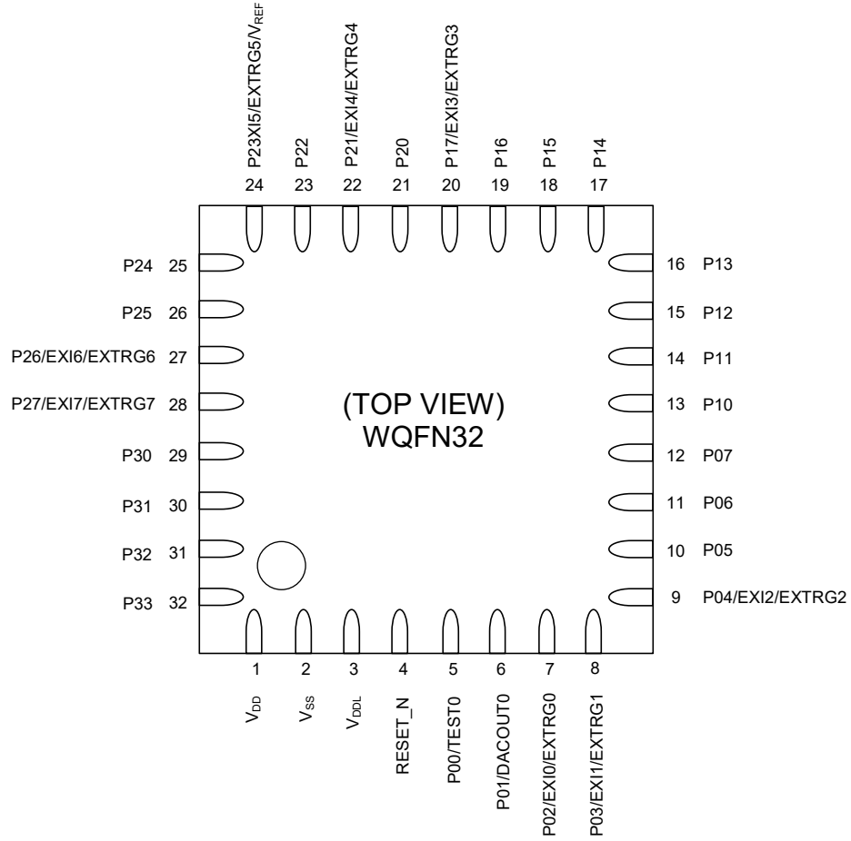
Figure 8 Pin Layout of 32pin WQFN Package
