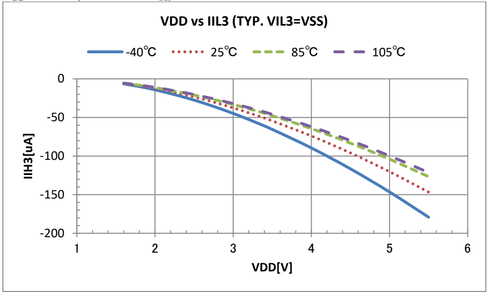
Pull-up resistor
