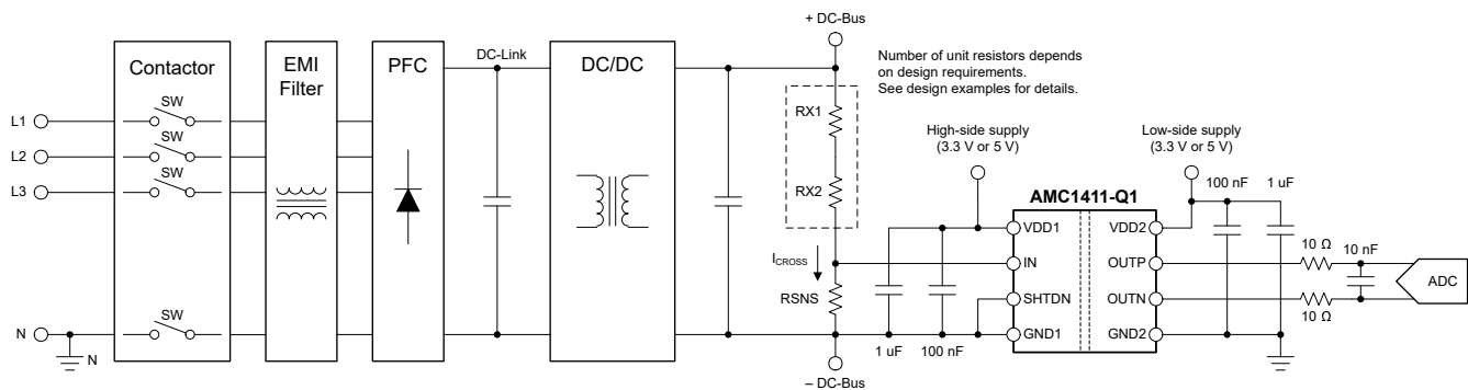
Figure 8-1. Using the AMC1411-Q1 for DC Bus Voltage Sensing in an OBC
