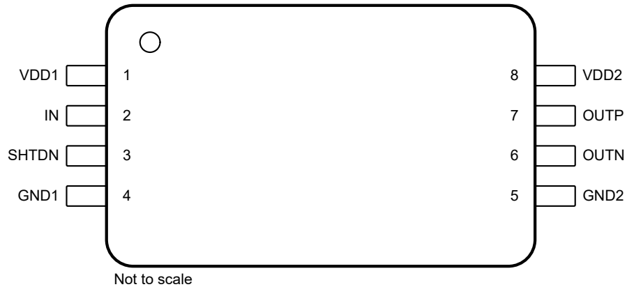
Figure 5-1. DWL Package, 8-Pin SOIC (Top View)
