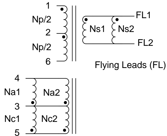
Figure 22. Transformer Schematic
