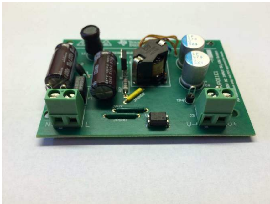
Figure 1. UCC28742EVM-001
