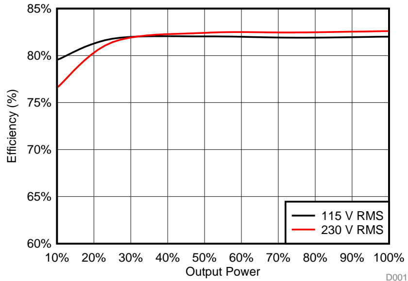
Figure 4. Efficiency
