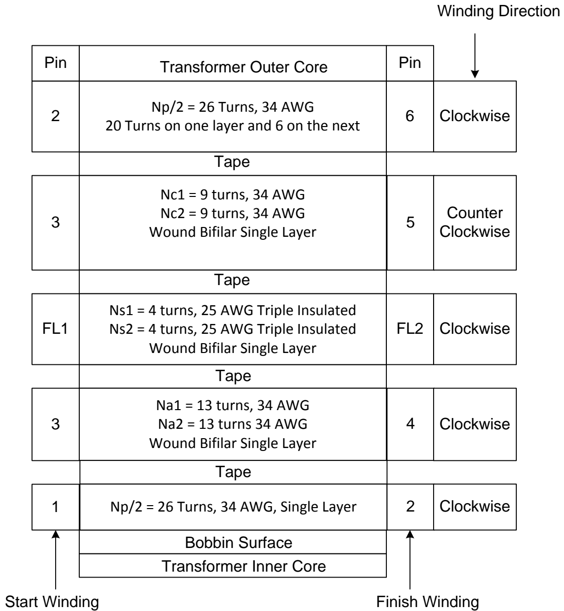
Figure 23. Transformer Winding Structure
