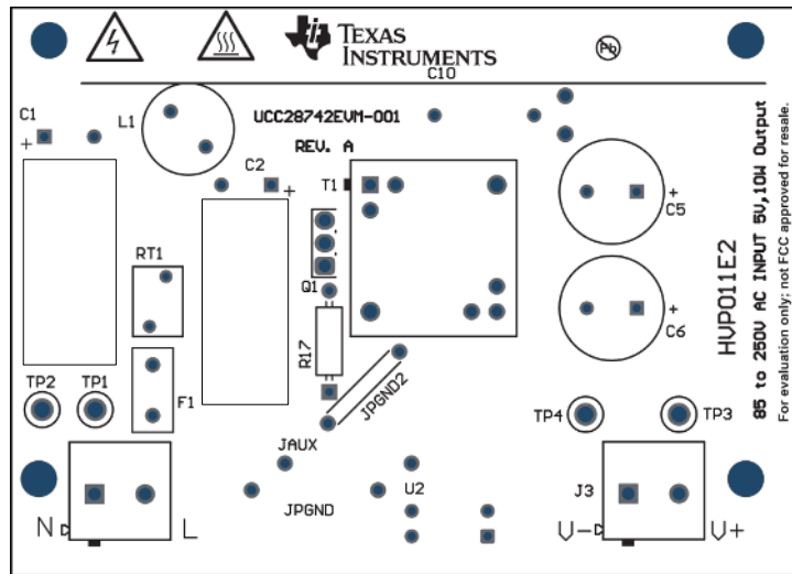
Figure 24. EVM Assembly (Top View)
