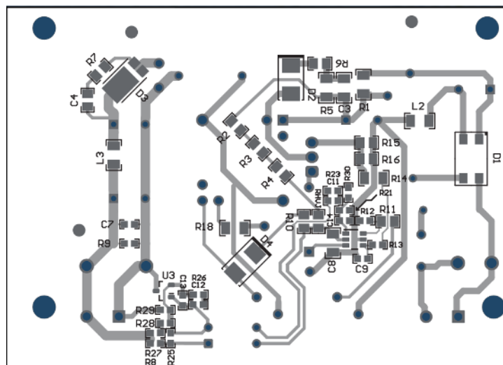
Figure 25. EVM Assembly/Layout (Bottom View)
