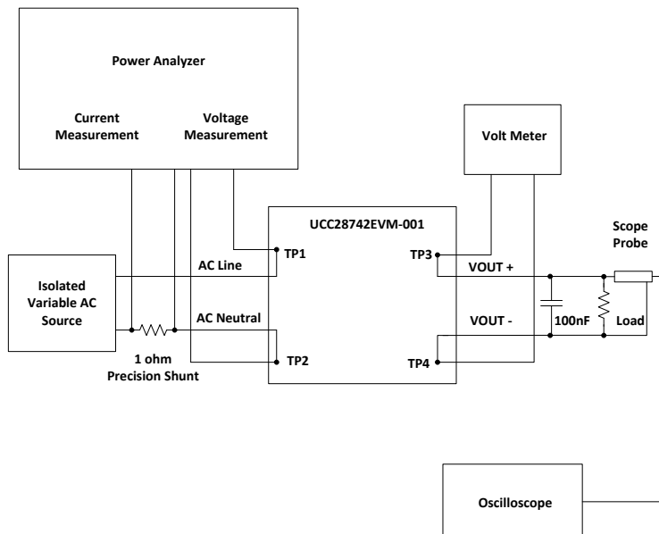
Figure 3. UCC28742EVM-001 Test Setup Diagram
