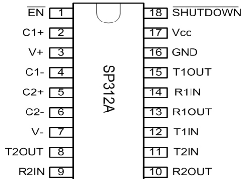
18 pin WSOIC
