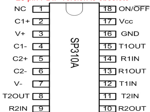
18 pin WSOIC
