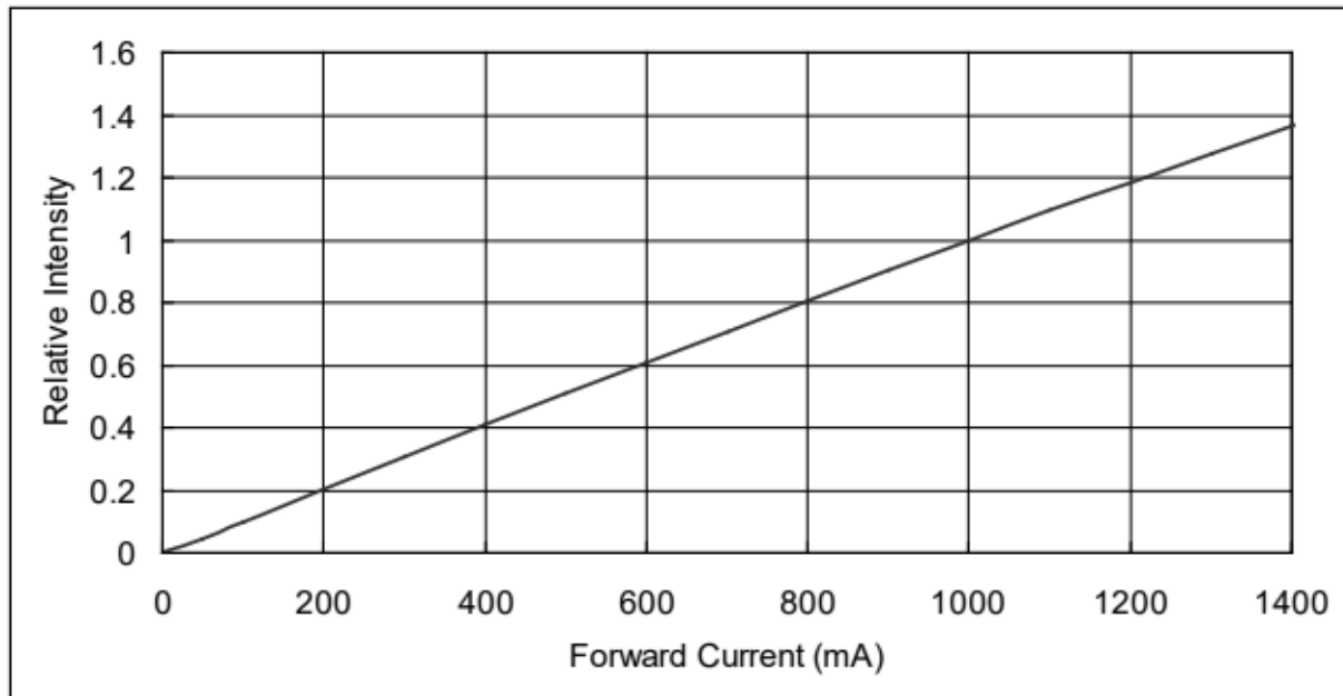
Relative Intensity vs. Forward Current
