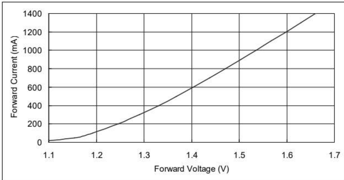
Forward Current vs. Forward Voltage
