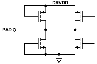
Figure 70. Digital Output
