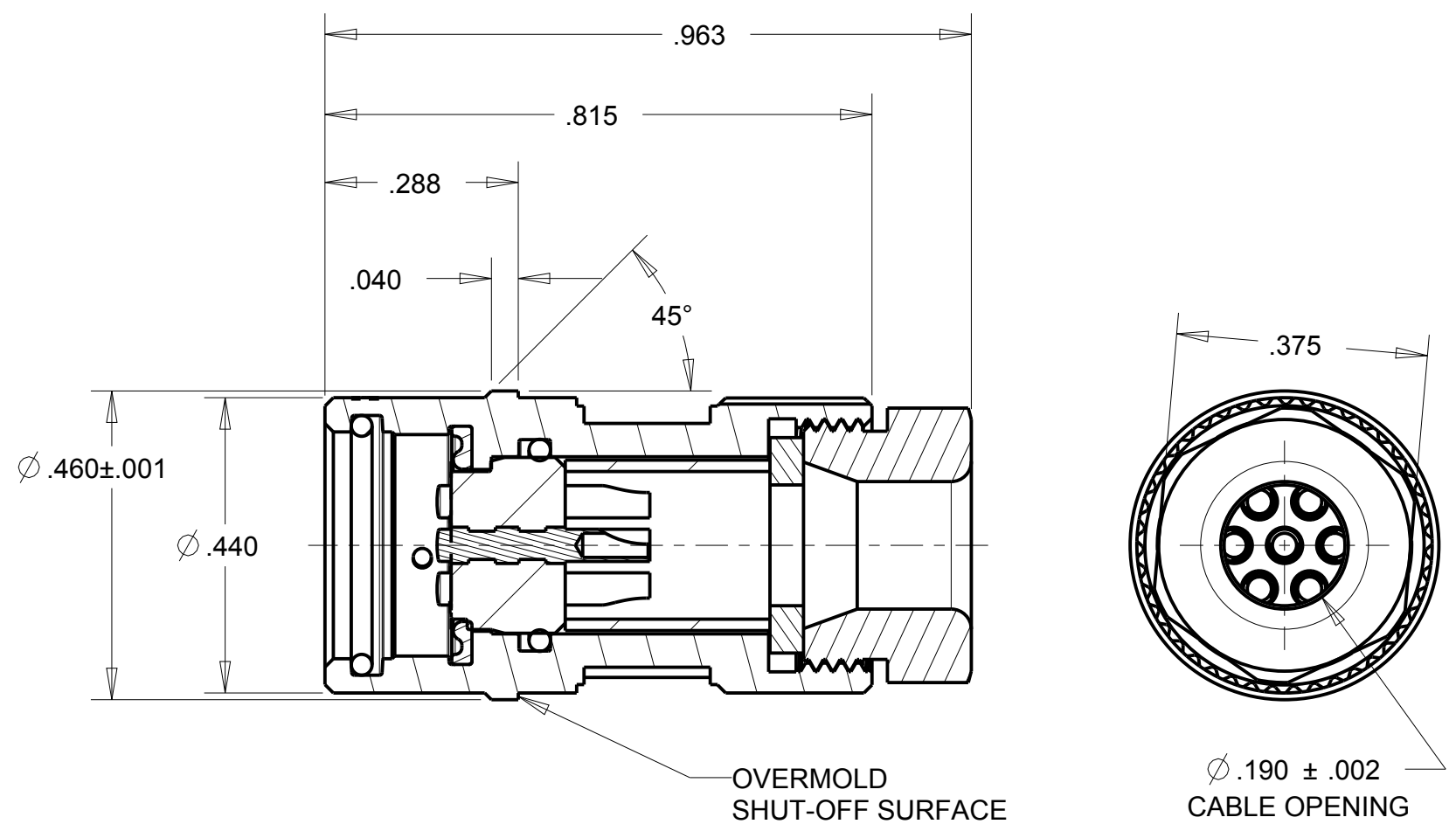
SECTION Z-Z
