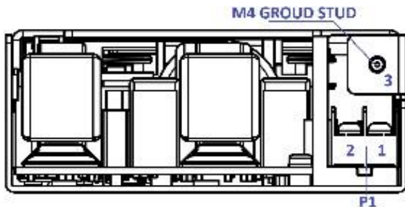
Figure 2. Front View - ABC1200-1T24-UCF Model
