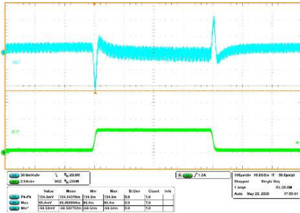
Figure 8-14. Transient Response 0.3 to 2.7 A with Slew Rate of 0.25 A/μs
