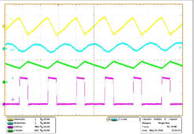
Figure 8-9. Steady State Waveforms, I_{OUT} = 3 \text{ A}
