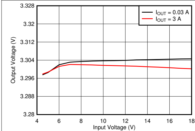
Figure 8-4. Line Regulation
