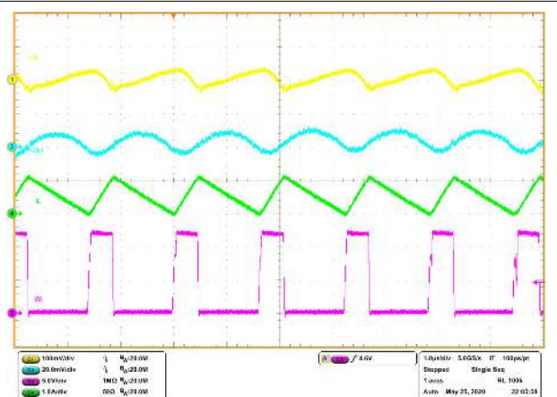
Figure 8-7. Steady State Waveforms, I_{OUT} = 0.5\text{ A}
