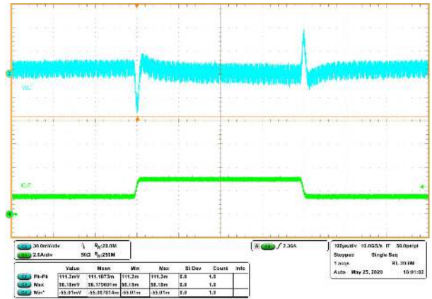
Figure 8-15. Transient Response 1.5 to 3 A with Slew Rate of 0.25 A/μs
