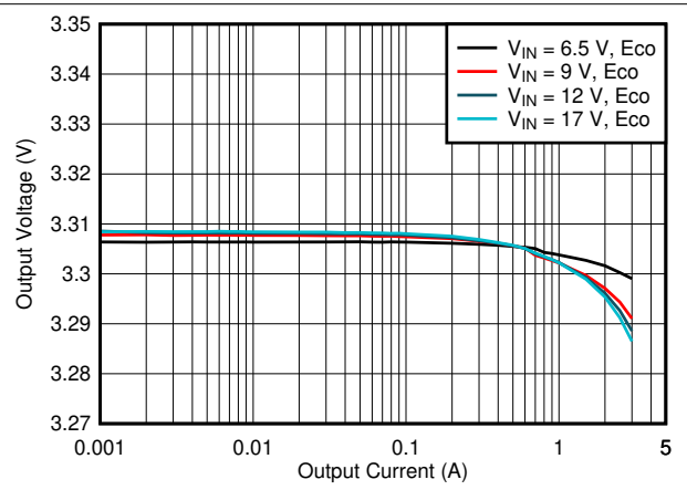
Figure 8-3. Load Regulation
