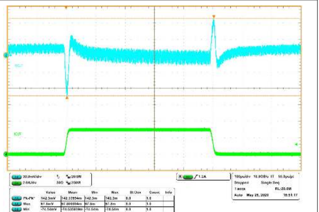
Figure 8-13. Transient Response 0.03 to 3 A with Slew Rate of 0.25 \text{ A}/\mu\text{s} (FCCM)
