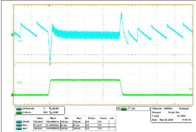
Figure 8-10. Transient Response 0 to 3 A with Slew Rate of 0.25 \text{ A}/\mu\text{s} (Eco-Mode)
