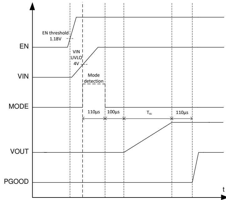
Figure 7-1. Power-Up Sequence
