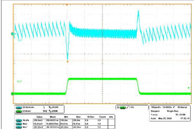
Figure 8-12. Transient Response 0.03 to 3 A with Slew Rate of 0.25 \text{ A}/\mu\text{s} (Eco-Mode)
