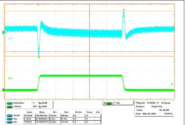
Figure 8-11. Transient Response 0 to 3 A with Slew Rate of 0.25 \text{ A}/\mu\text{s} (FCCM)
