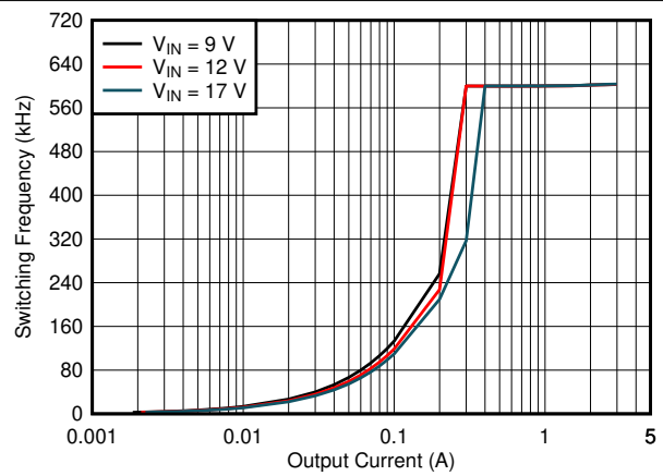
Figure 6-12. Switching Frequency vs Output Current, V_{OUT} = 3.3\text{ V} , L = 3.3\text{ }\mu\text{H}
