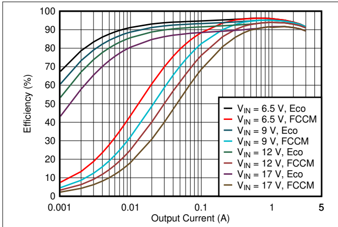
Figure 8-2. Efficiency
