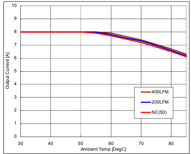
Fig.2: Output current vs. ambient temperature and air velocity at 5.0Vin, 2.5V out
