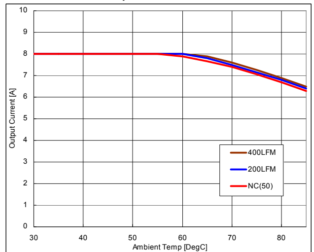
Fig.6: Output current vs. ambient temperature and air velocity at 5.0Vin, 1.0V out
