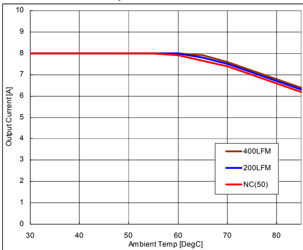
Fig.5: Output current vs. ambient temperature and air velocity at 5.0Vin, 1.2V out
