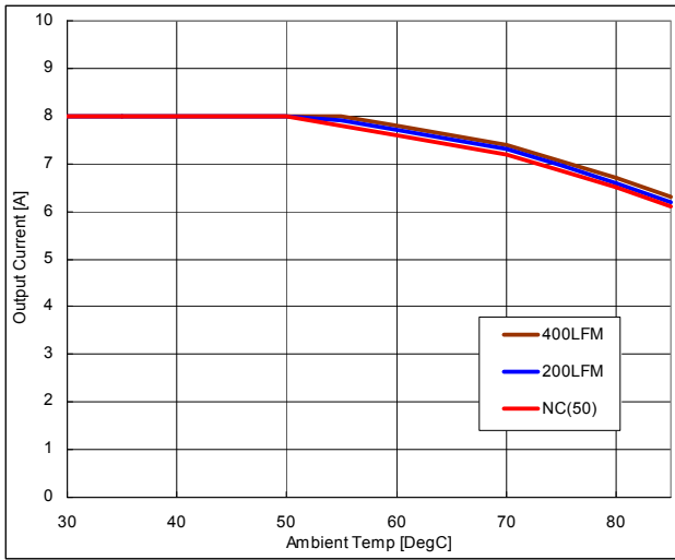
Fig.1: Output current vs. ambient temperature and air velocity at 5.0Vin, 2.75V out
