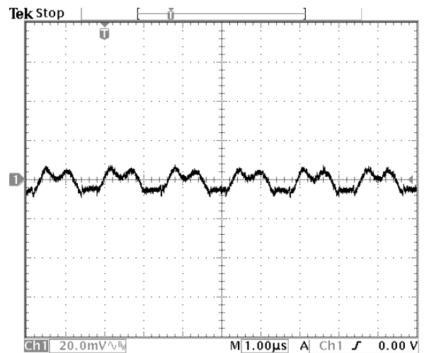
Fig.20: Output ripple and noise at 5.0Vin, 0.8V/8Aout
