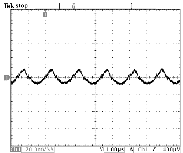
Fig.16: Output ripple and noise at 5.0Vin, 2.75V/8Aout
