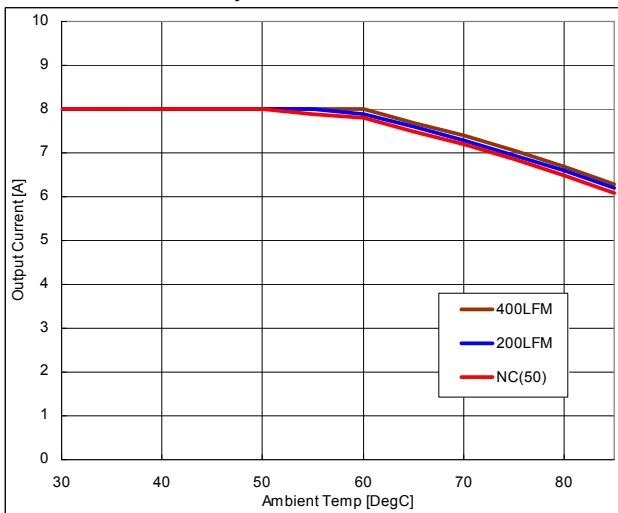
Fig.3: Output current vs. ambient temperature and air velocity at 5.0Vin, 1.8V out
