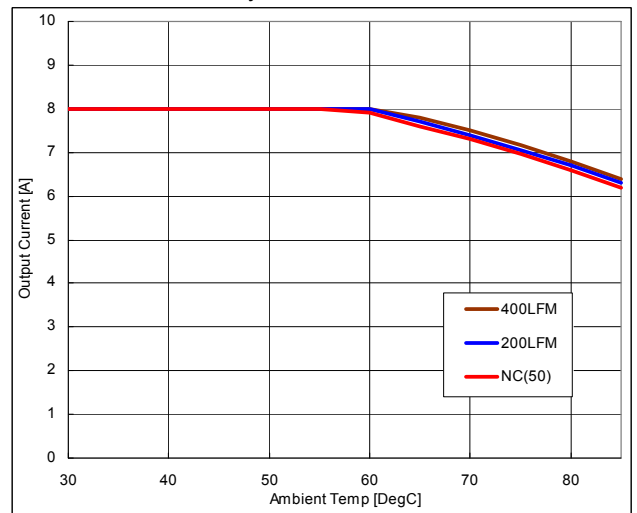
Fig.4: Output current vs. ambient temperature and air velocity at 5.0Vin, 1.5V out
