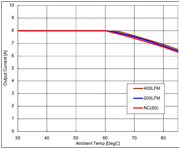
Fig.7: Output current vs. ambient temperature and air velocity at 5.0Vin, 0.8V out
