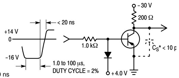
Figure 2. Turn–Off Time
